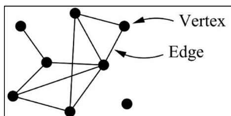
Figure 4. A network with 8 nodes and 10 edges
