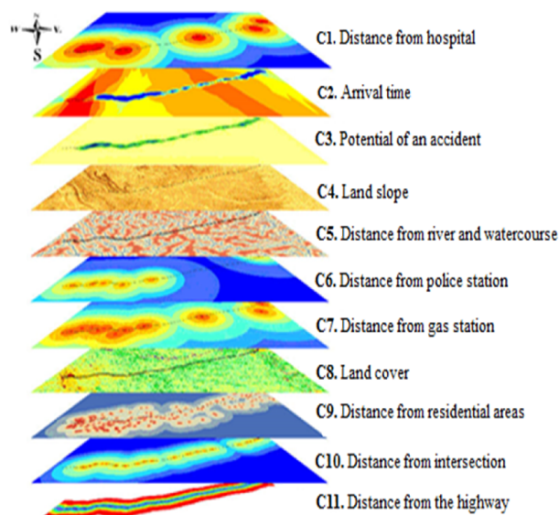
Figure 2. Classified layers
